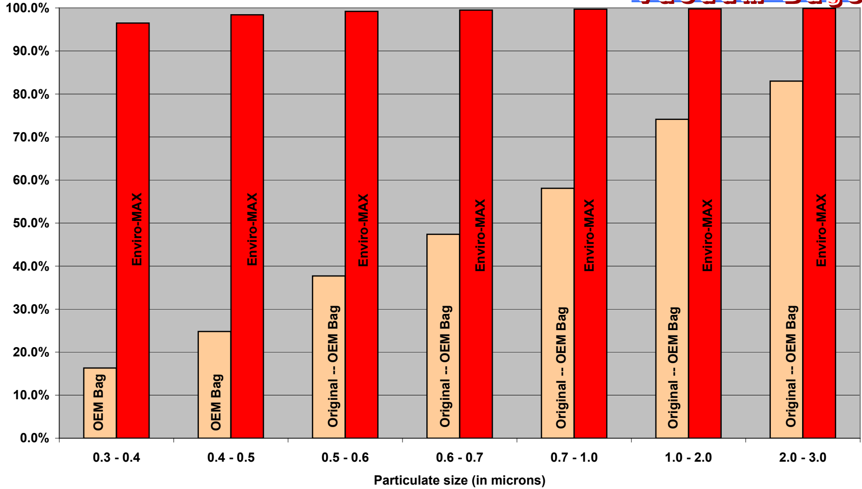
Enviro-MAX Filtering Efficiency as compared to "OEM" bags
